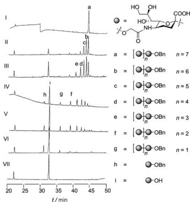
Figure 2. The products obtained from the hydrolysis of \alpha -(2 \rightarrow 5)Neu5Gc octamer 38 by neuraminidase were analyzed by CE at different times intervals (I, 0 min; II, 1 h; III, 90 mins; IV, 3 h; V, 4 h; VI, 6 h; VII, 1 day). Peaks a–h were assigned to octamer, heptamer, hexamer, pentamer, tetramer, trimer, dimer (2 \rightarrow 5)Neu5Gc-2-OBn, and monomer Neu5Gc-2-OBn respectively, peak i was monomer Neu5Gc-2-OH.
